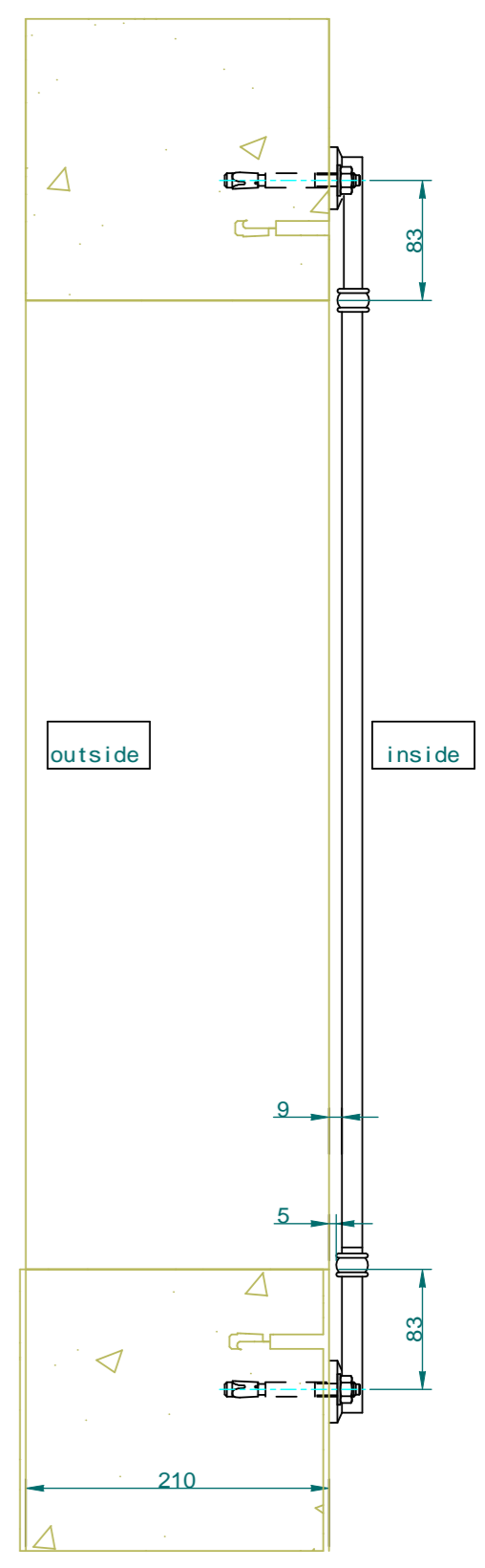
SIDE VIEW 1:5
