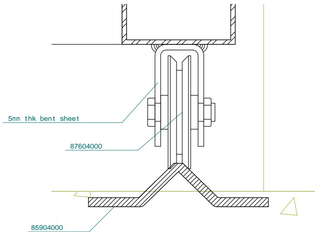
wheel detail scale 1:2
