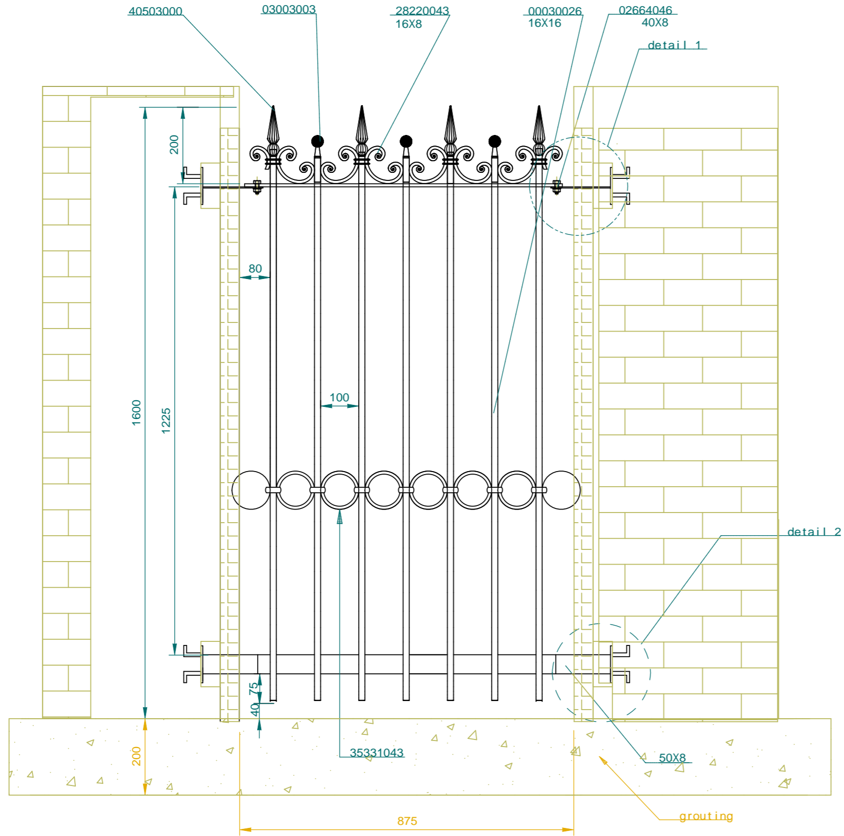
Elevation 1:10
