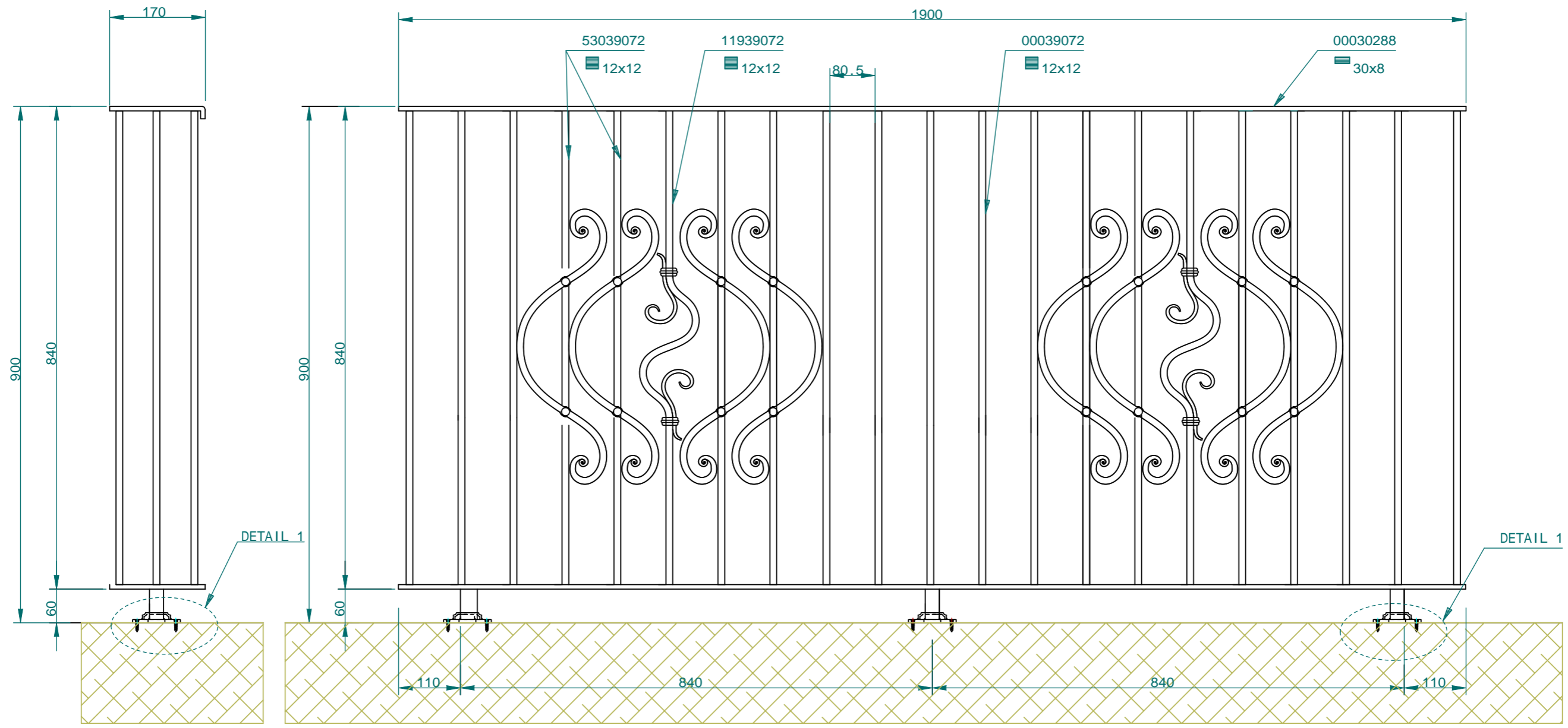
ELEVATION 3-1 & 3-3 scale 1:8
