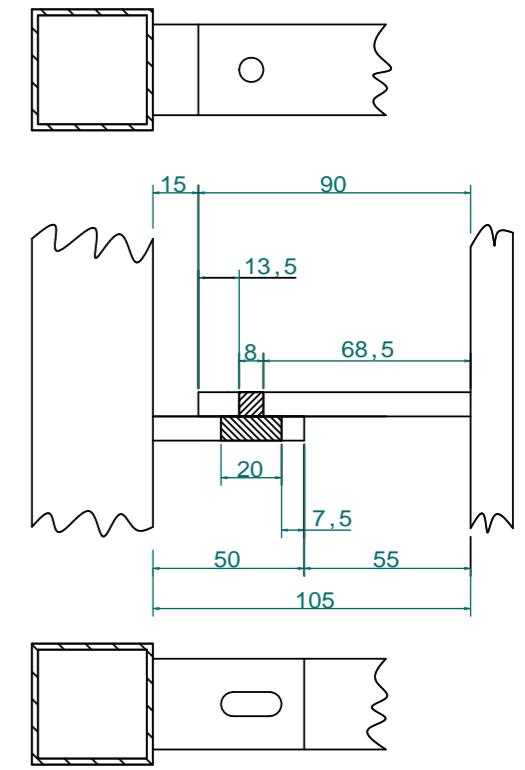
DETAL A SCALE 1:4
