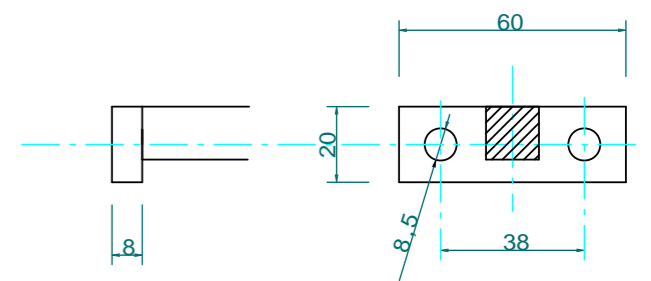
DETAIL A 1:2
